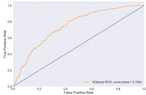
Fig. 1 ROC curve of the XGBoost classifier on the Test set.
