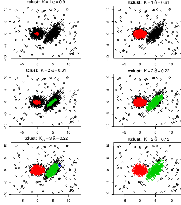
Fig. 1 The application of Algorithm 1 to a 2- dimensional simulated composed by K = 2 clusters and a proportion of contaminating points equal to 0.10.
